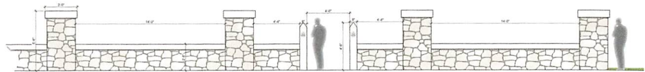
SAGAMORE GREENSPACE WALL AND PEDESTAIN ENTRANCE
