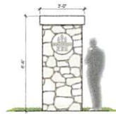
TYPICAL SINGLE COLUMN SIGNATURE ENTRY
